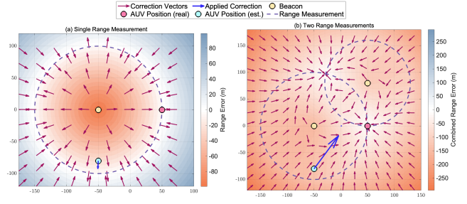
Fig. 3: EKF linearized measurement model: (Left) Single range update may result in suboptimal correction; (Right) Two range updates constrain the solution to two possible estimates, improving accuracy.
